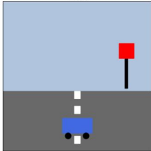
Illumination i(x,y)
