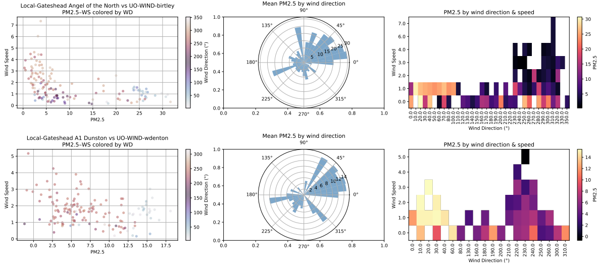
Figure 14: Scatter plots of PM2.5 concentration to wind speed coloured by wind direction, rose plots of PM2.5 concentration to wind direction, and binned plots of wind speed and direction coloured by PM2.5 concentration for the closest Local sensors to UO wind sensors in Birtley and West Denton.
