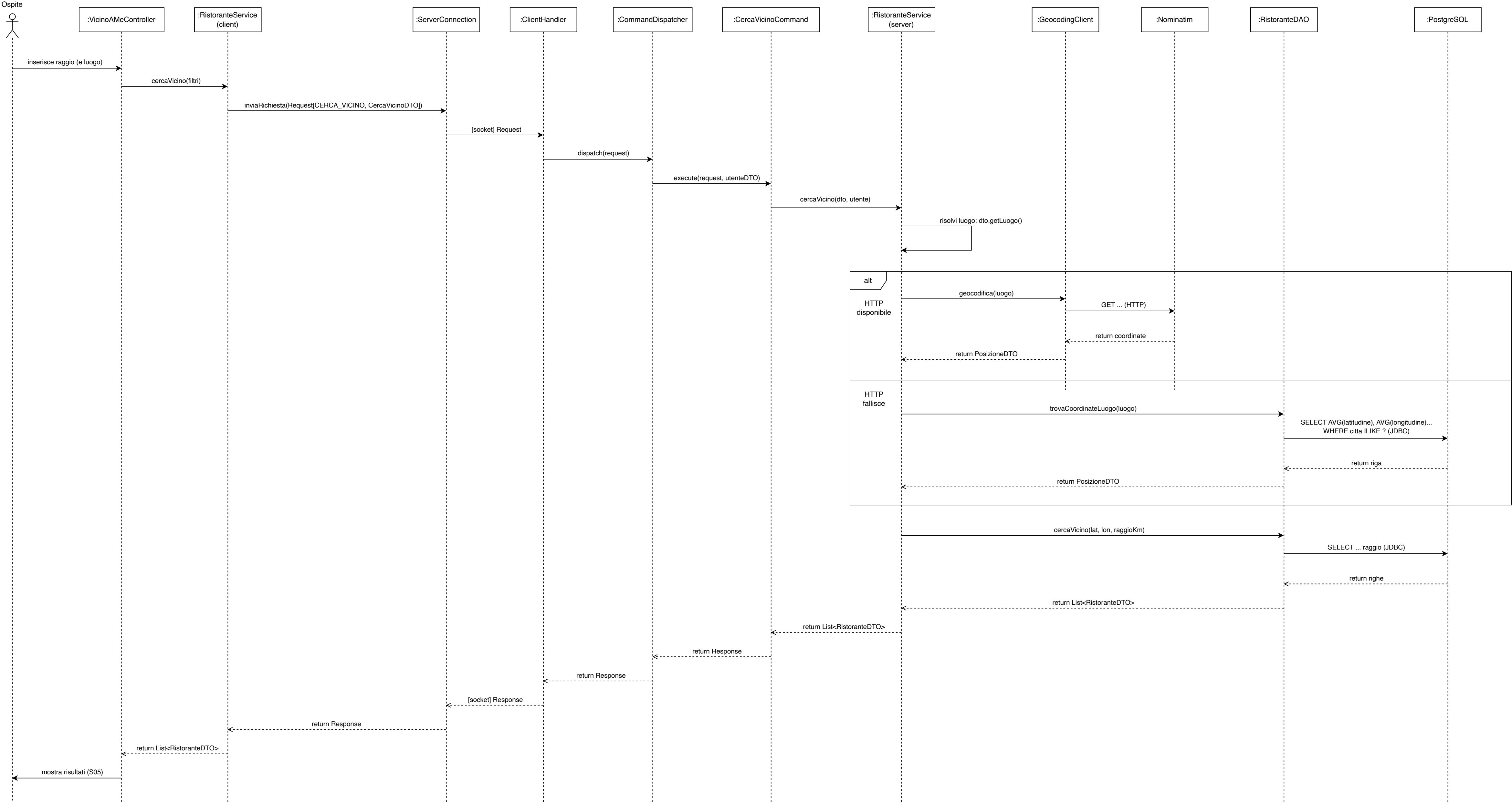
Sequence Diagram — Cerca Vicino
