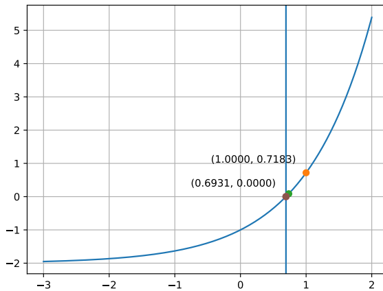
Fig. 2.2.7.1. Convergence of the Newton-Raphson method to x = \ln 2
