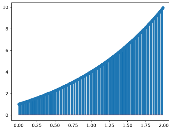
Fig. 1.2.3.1. Euler's Forward Difference Simulation of Bacterial Growth
