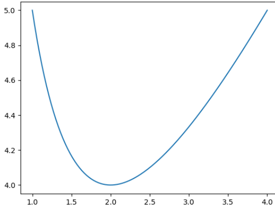
Fig. 1.2.4.1. Plot of f(x) = x + \frac{4}{x} indicating the minimum at (2, 4)
