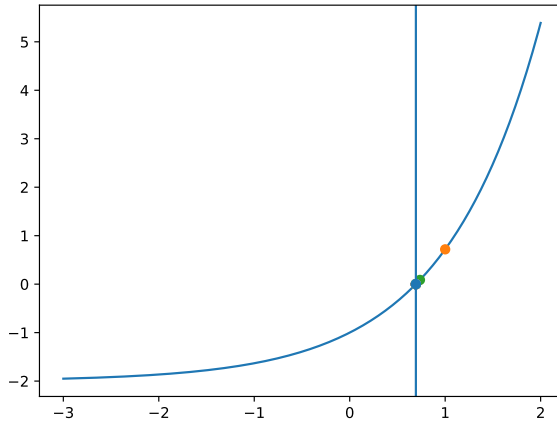
Fig. 1.2.5.1. Convergence of the Newton-Raphson method to x = \ln 2
