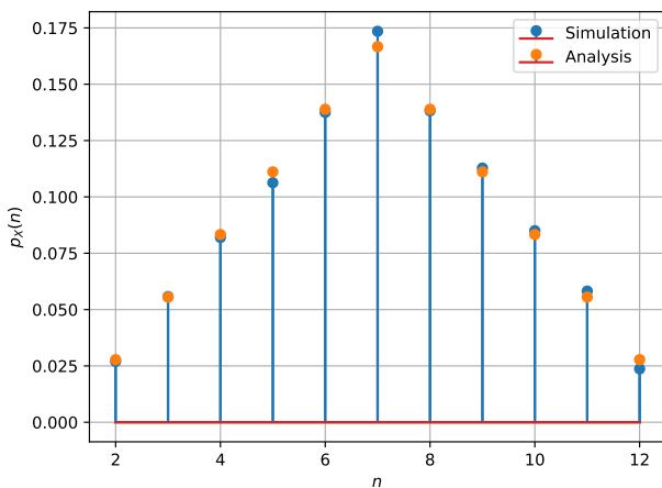
Fig. 1.2.7.1. PMF of the sum of two fair dice: Simulation vs Analysis
