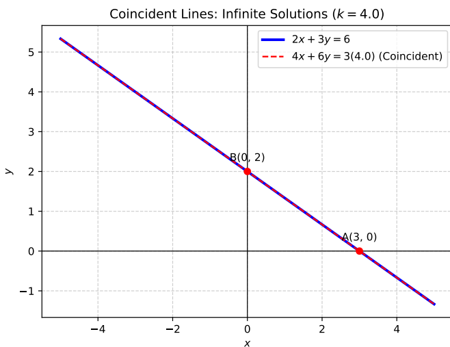
Fig. 1.2.6.1. Coincident lines representing infinitely many solutions at k = 4
