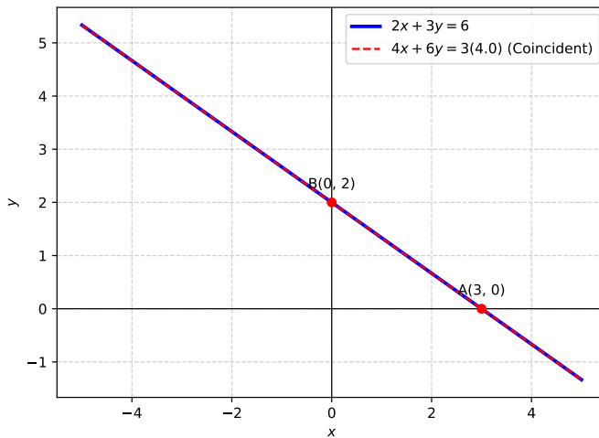
Coincident Lines: Infinite Solutions ( k = 4.0 )
