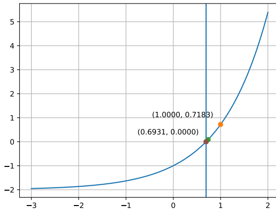
Fig. 2.2.5.1. Convergence of the Newton-Raphson method to x = \ln 2
