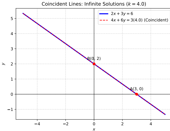
Fig. 2.2.6.1. Coincident lines representing infinitely many solutions at k = 4
