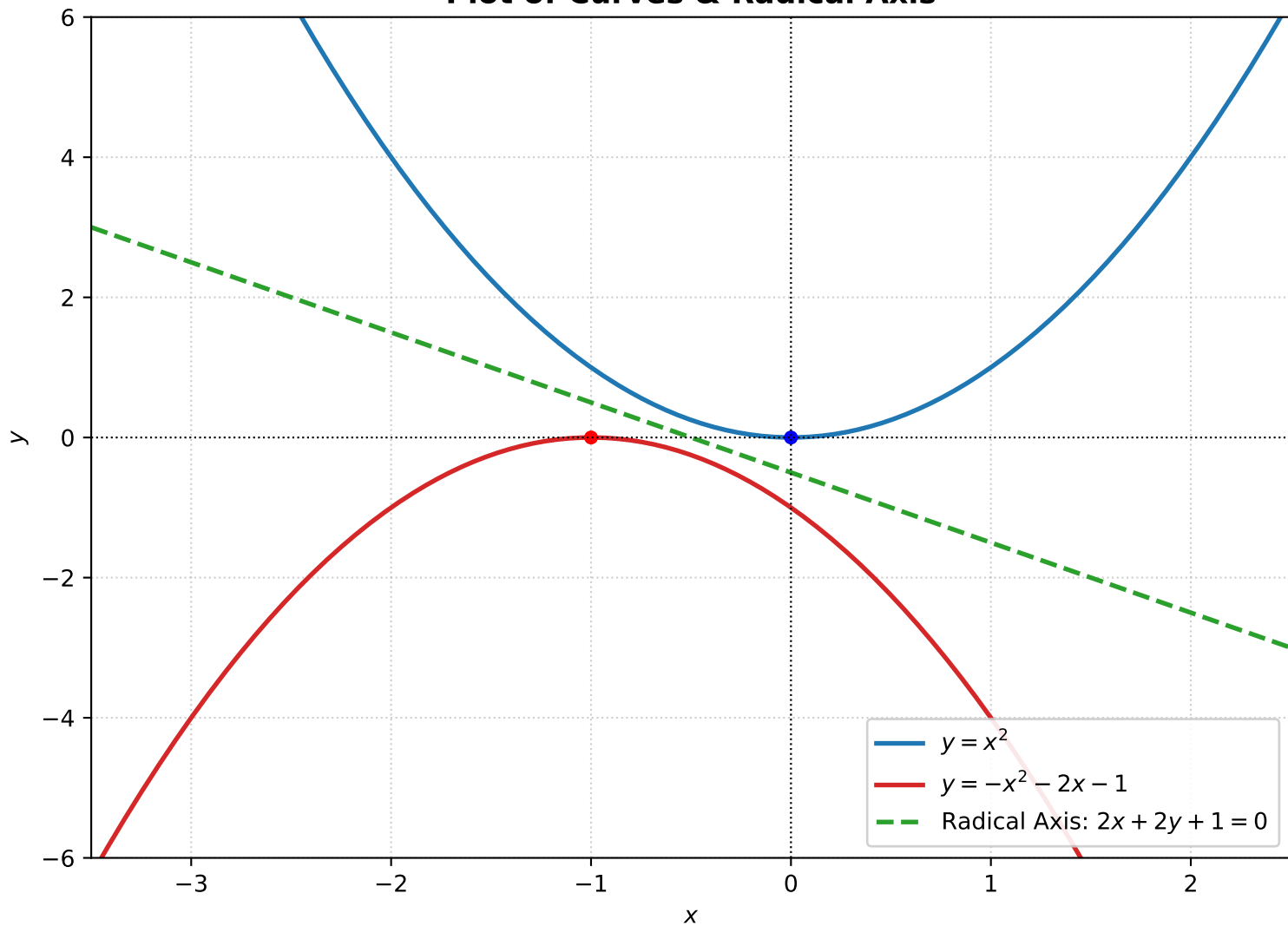
Plot of Curves & Radical Axis
