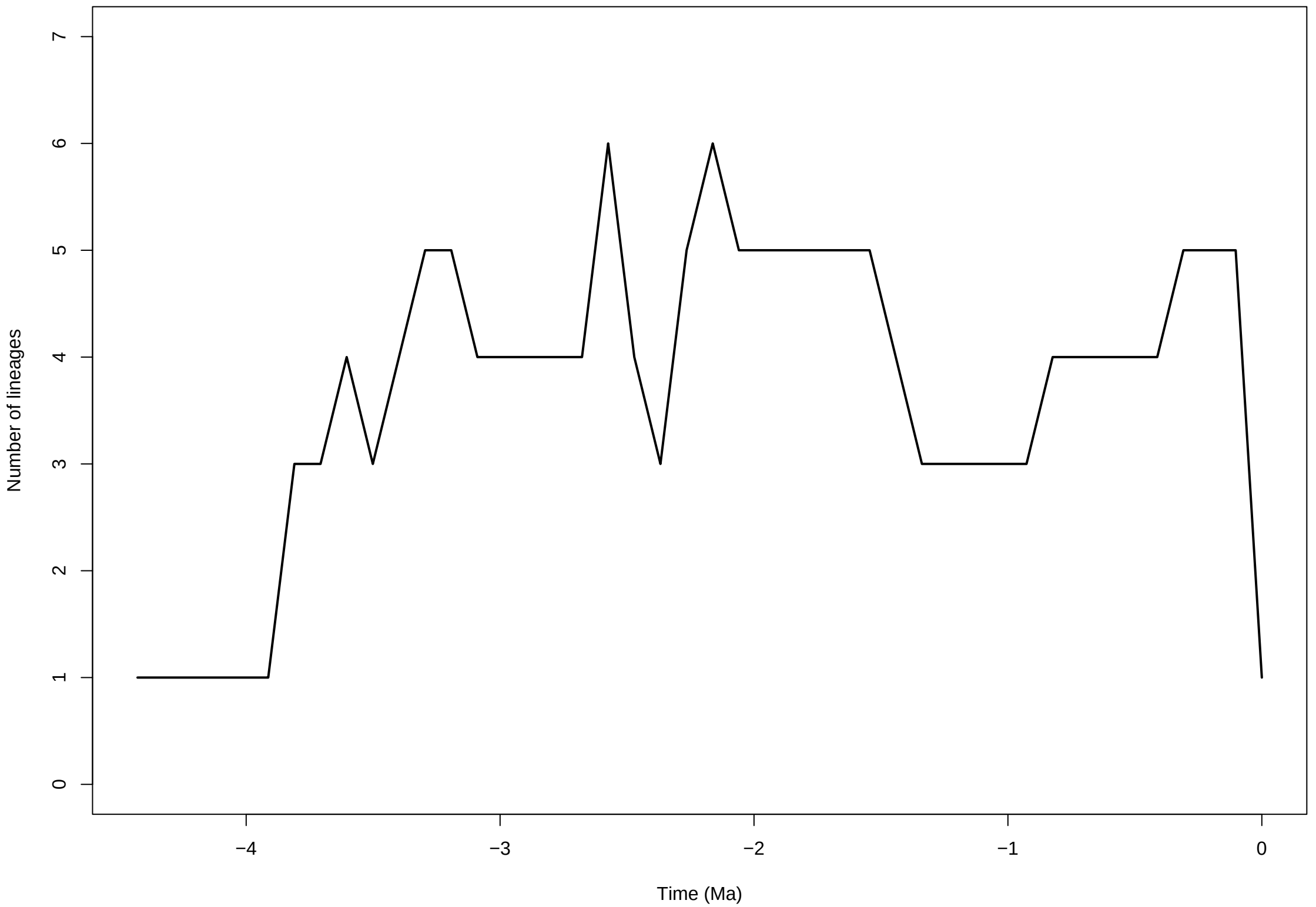
Range-through diversity through time
