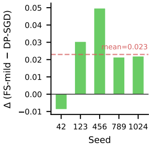
Combined Macro-F1
