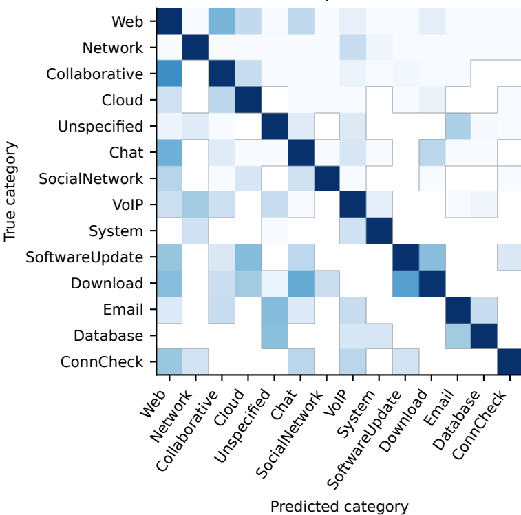
CNN1D / Sequential-SPLT-50
