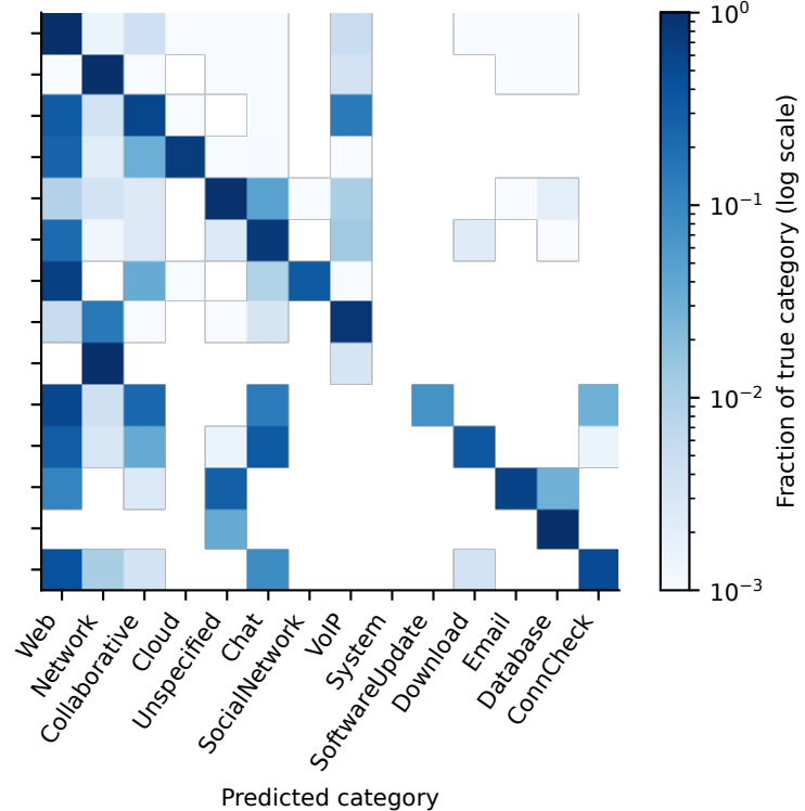
XGBoost / Flattened-SPLT-50
