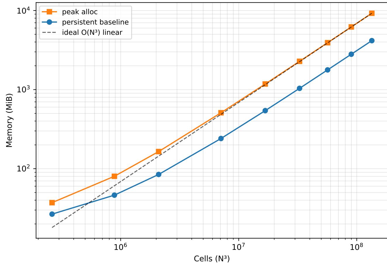
Log-log scaling — does peak grow linearly with N^3 ?
