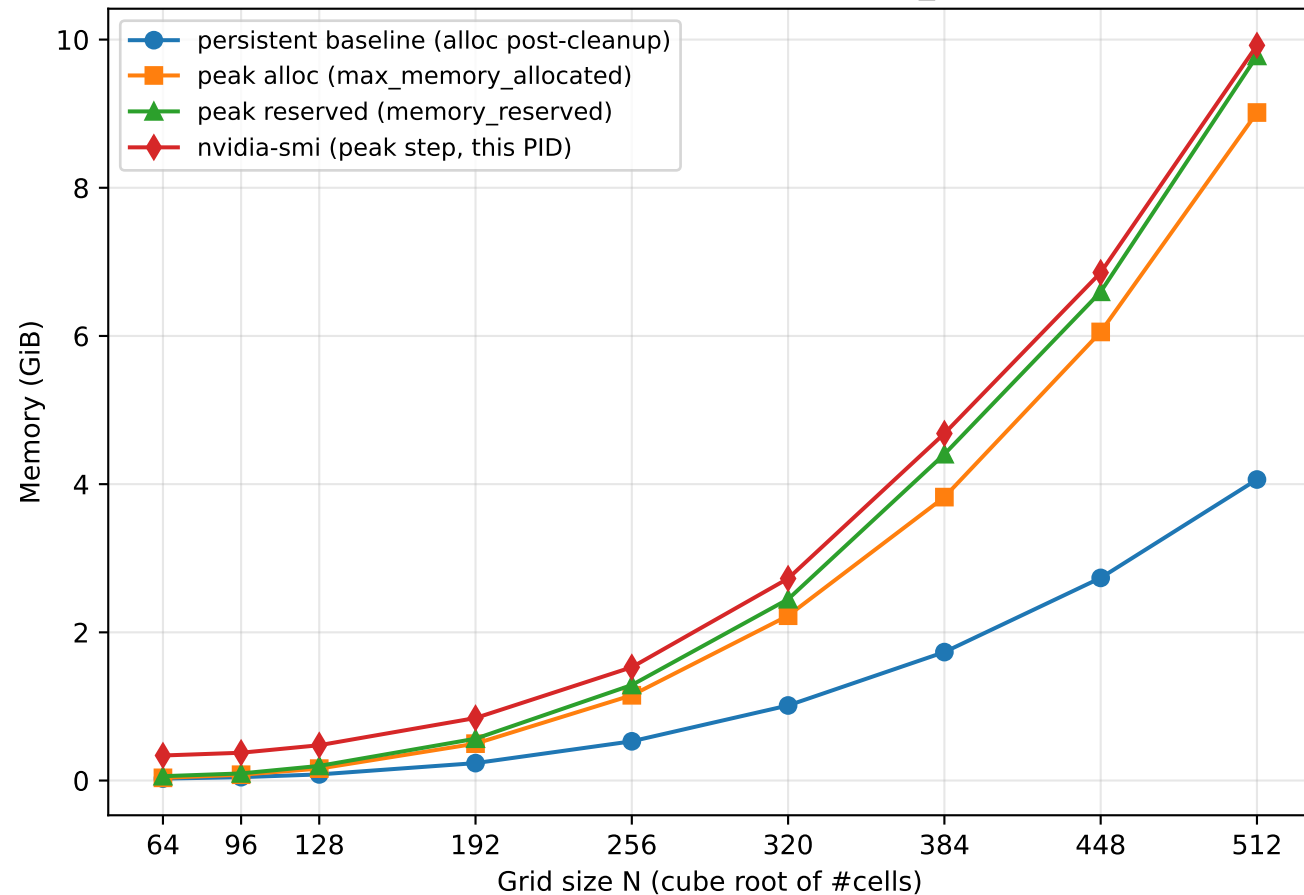
Peak memory vs grid size — mode=kernel, n_bodies=1, float32
