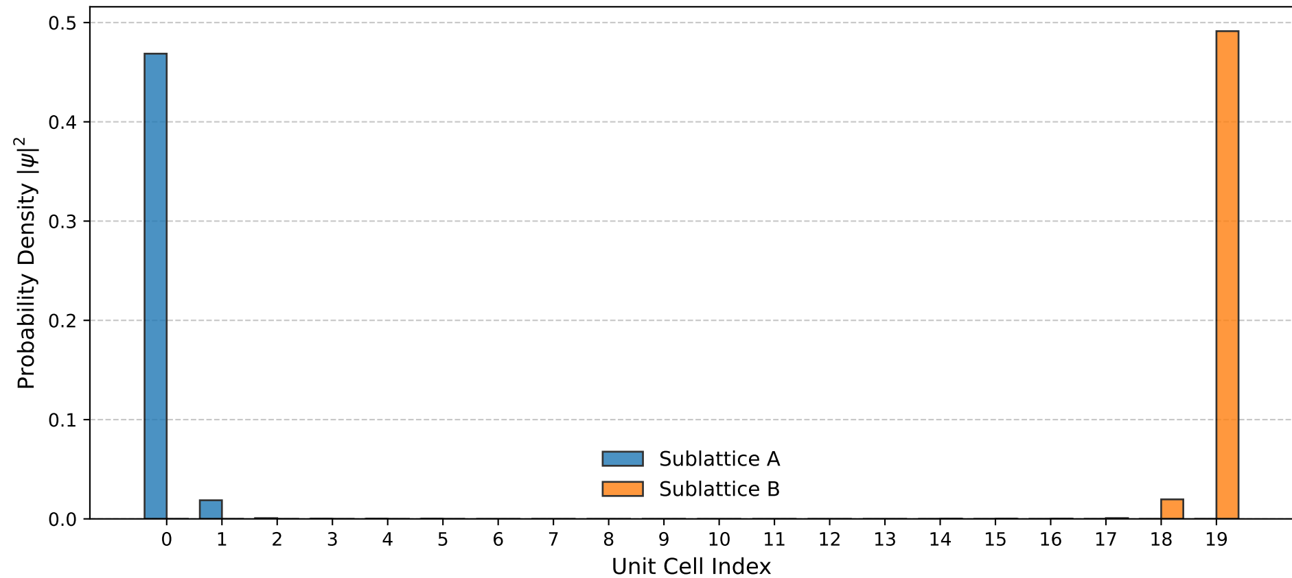
SSH State Probability Distribution ( \nu = 0.2 , w = 1.0 , N = 20 )
