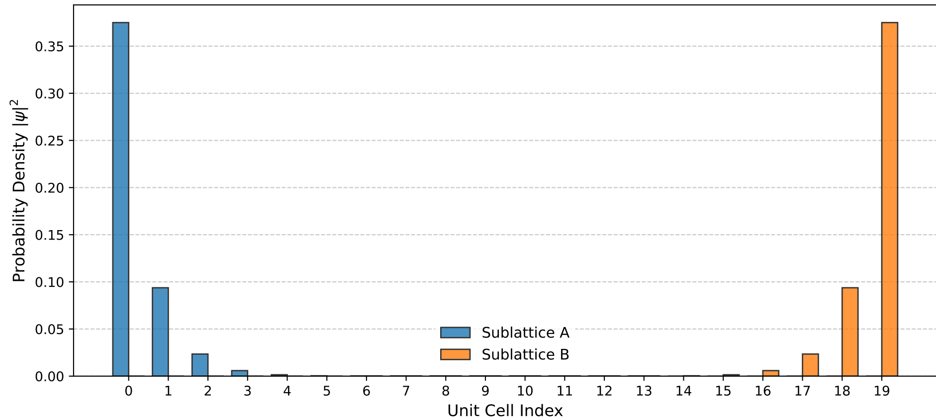
SSH State Probability Distribution ( v = 0.5 , w = 1.0 , N = 20 )
