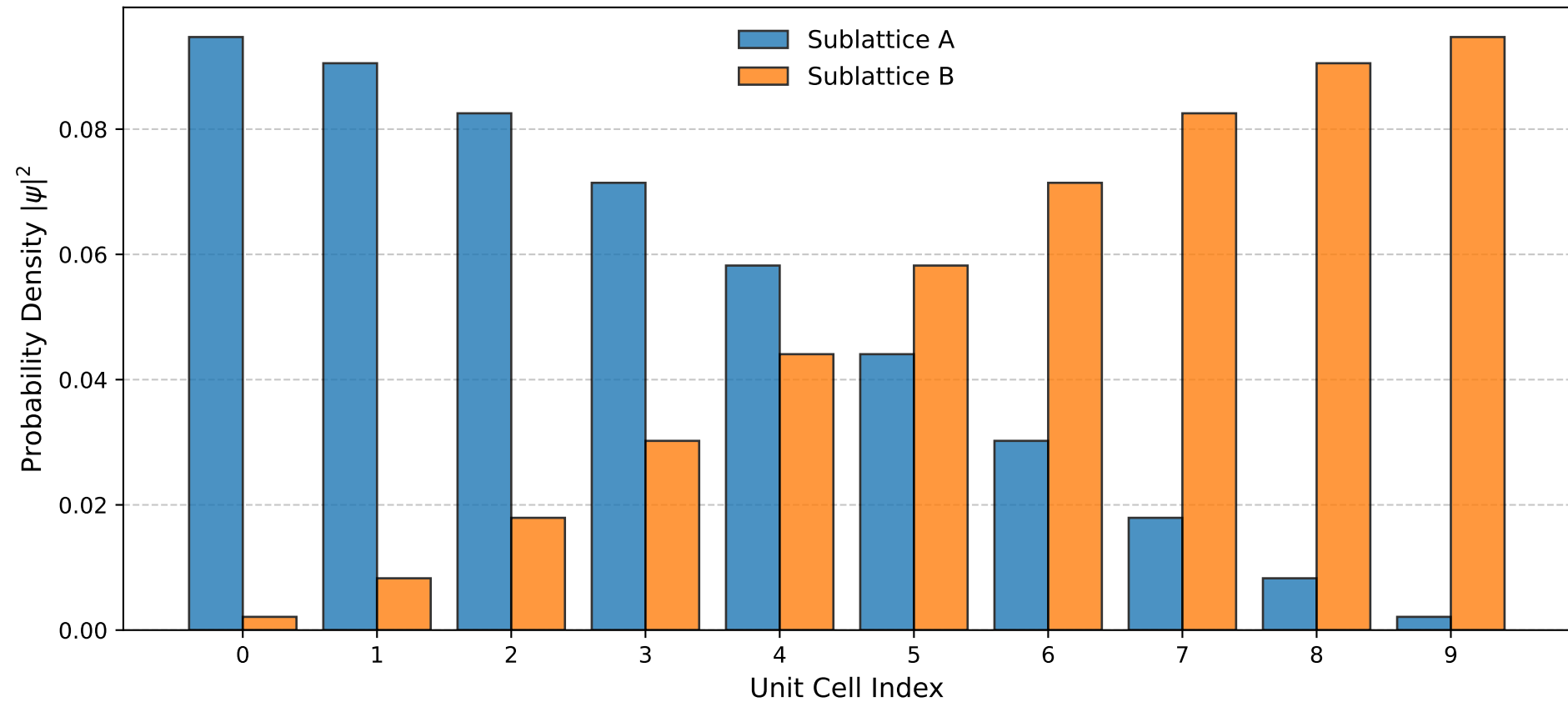
SSH State Probability Distribution ( v = 1.0 , w = 1.0 , N = 10 )
