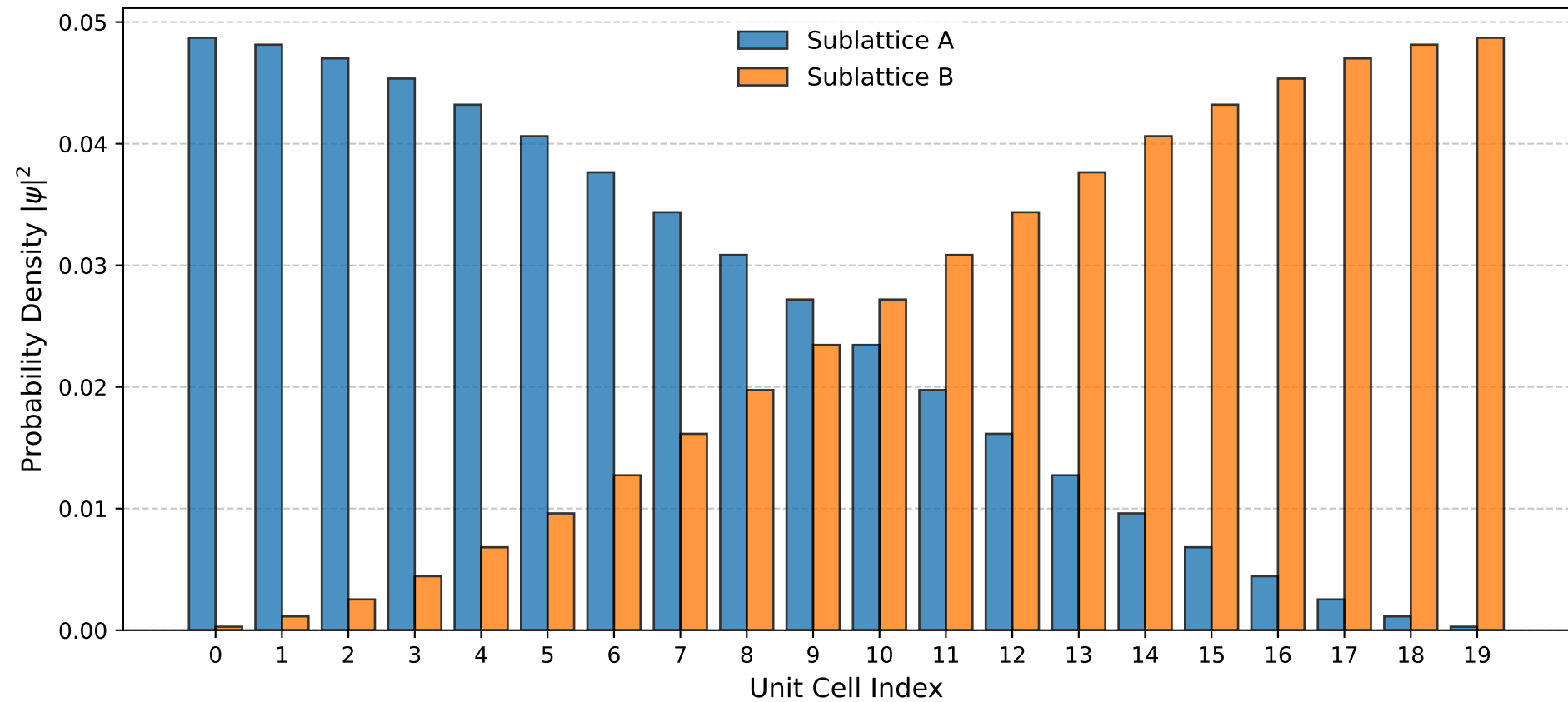
SSH State Probability Distribution ( v = 1.0 , w = 1.0 , N = 20 )
