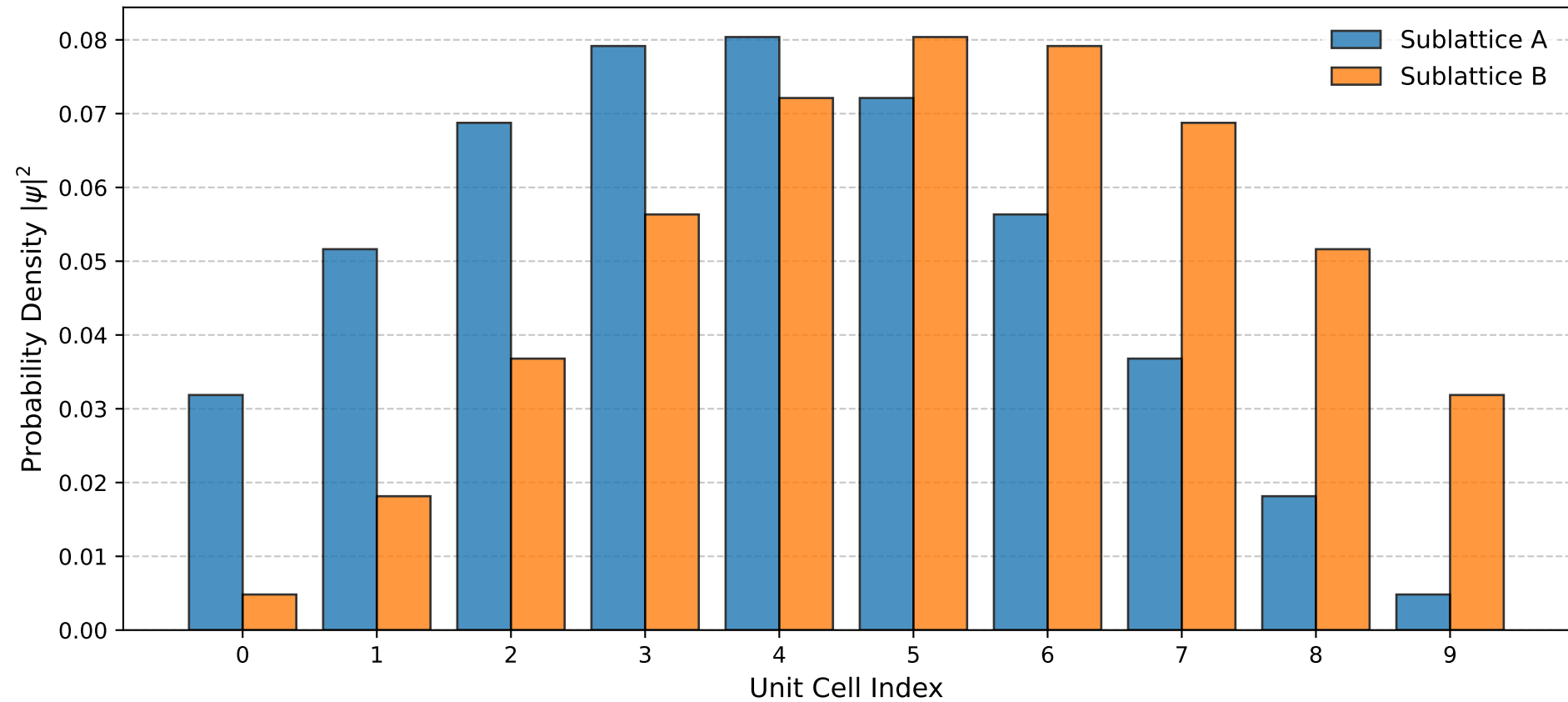
SSH State Probability Distribution ( \nu = 1.5 , w = 1.0 , N = 10 )
