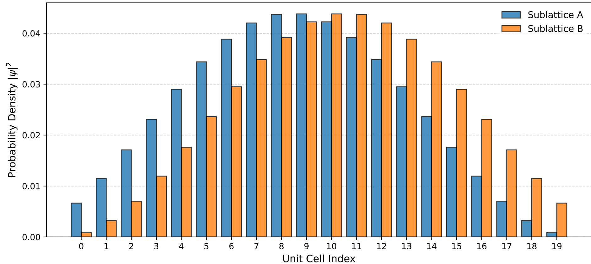
SSH State Probability Distribution ( v = 1.5 , w = 1.0 , N = 20 )
