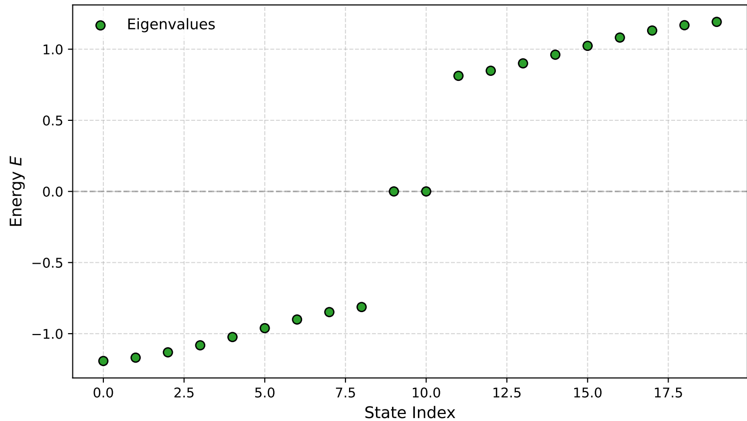
SSH Energy Spectrum ( \nu = 0.2 , w = 1.0 , N = 10.0 )
