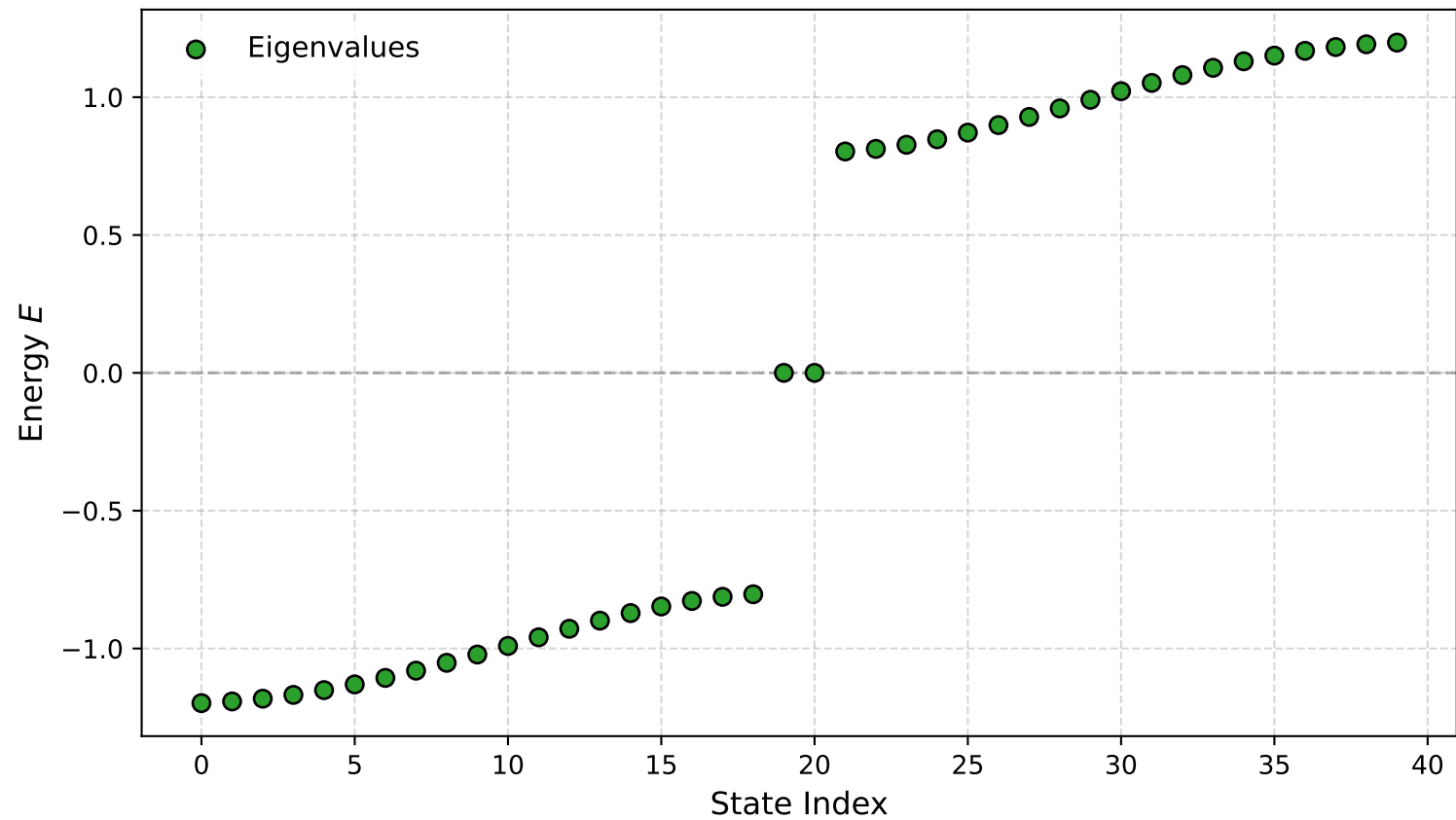
SSH Energy Spectrum ( \nu = 0.2 , w = 1.0 , N = 20.0 )
