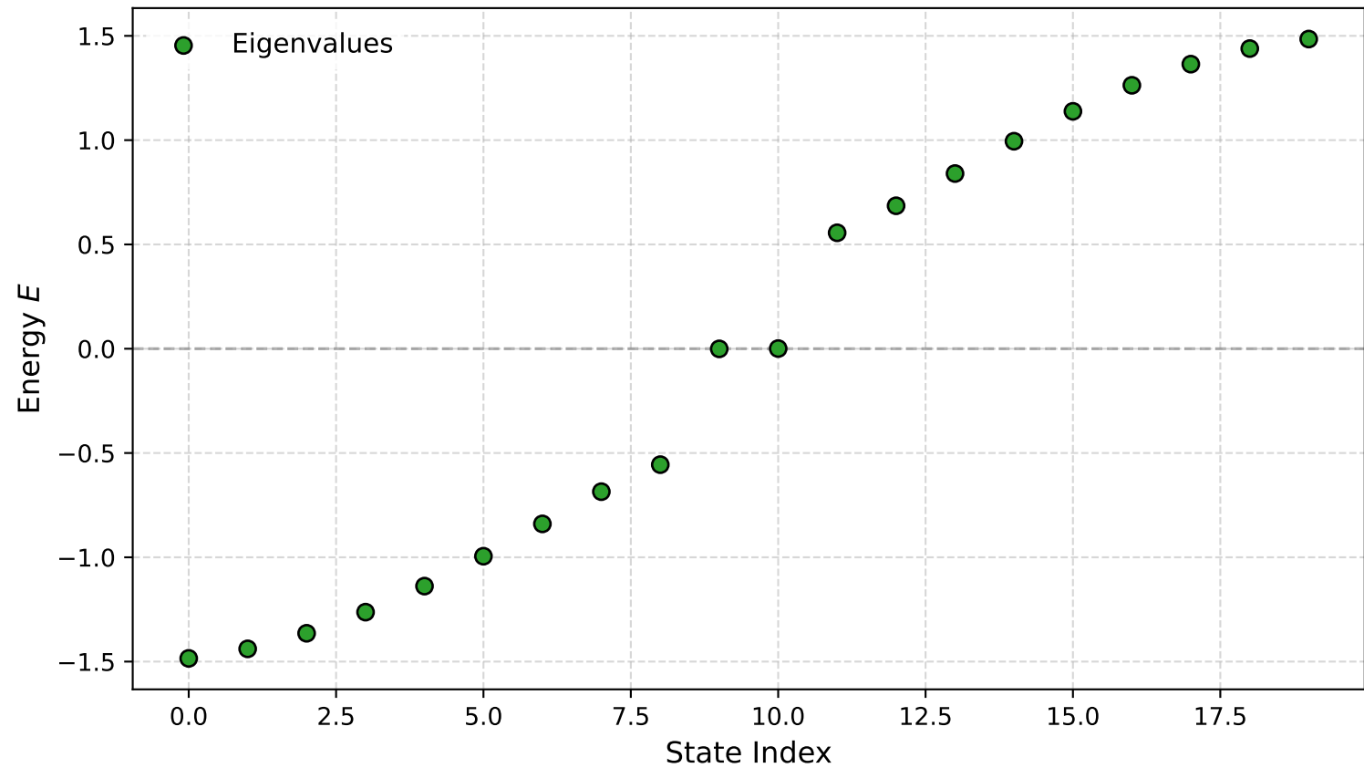
SSH Energy Spectrum ( v = 0.5 , w = 1.0 , N = 10.0 )
