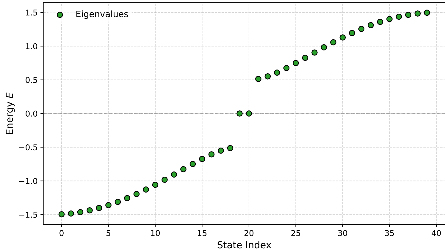
SSH Energy Spectrum ( \nu = 0.5 , w = 1.0 , N = 20.0 )
