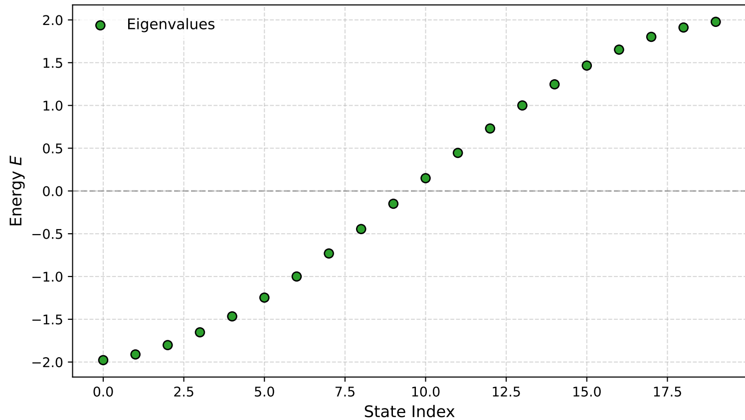
SSH Energy Spectrum ( \nu = 1.0 , w = 1.0 , N = 10.0 )
