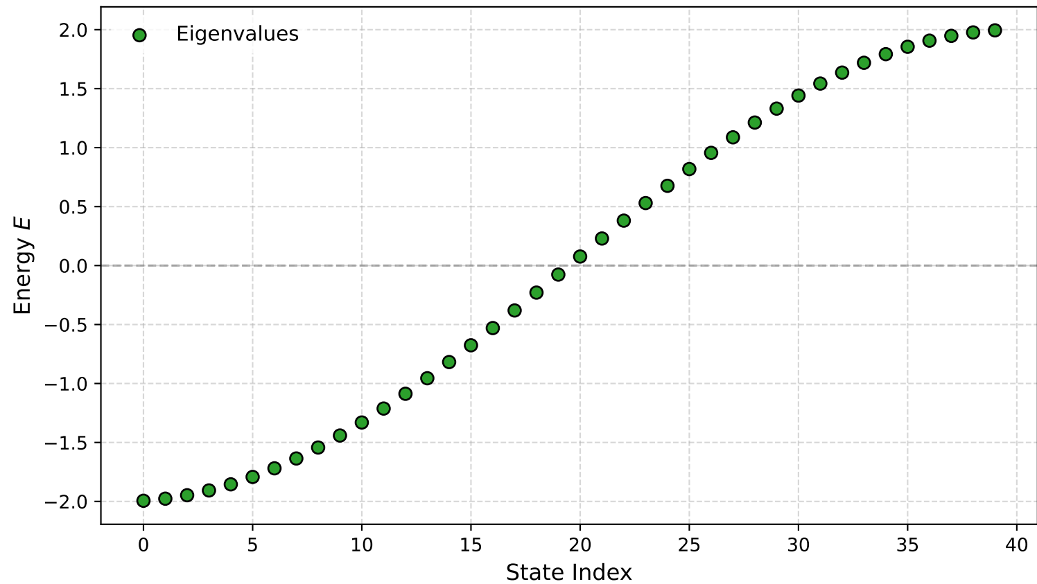
SSH Energy Spectrum ( v = 1.0 , w = 1.0 , N = 20.0 )
