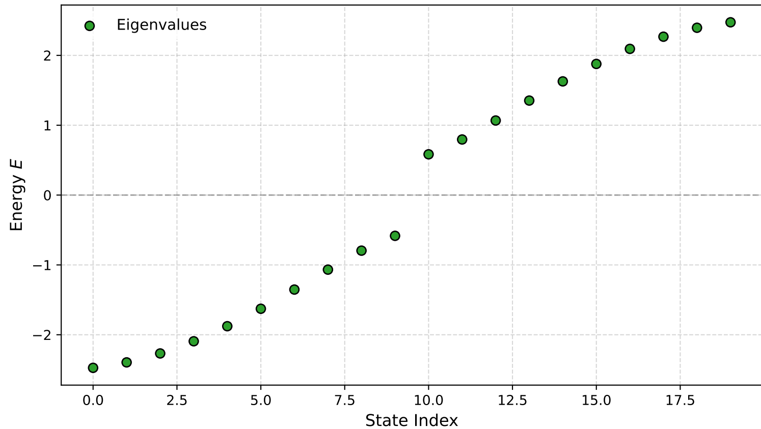
SSH Energy Spectrum ( \nu = 1.5 , w = 1.0 , N = 10.0 )
