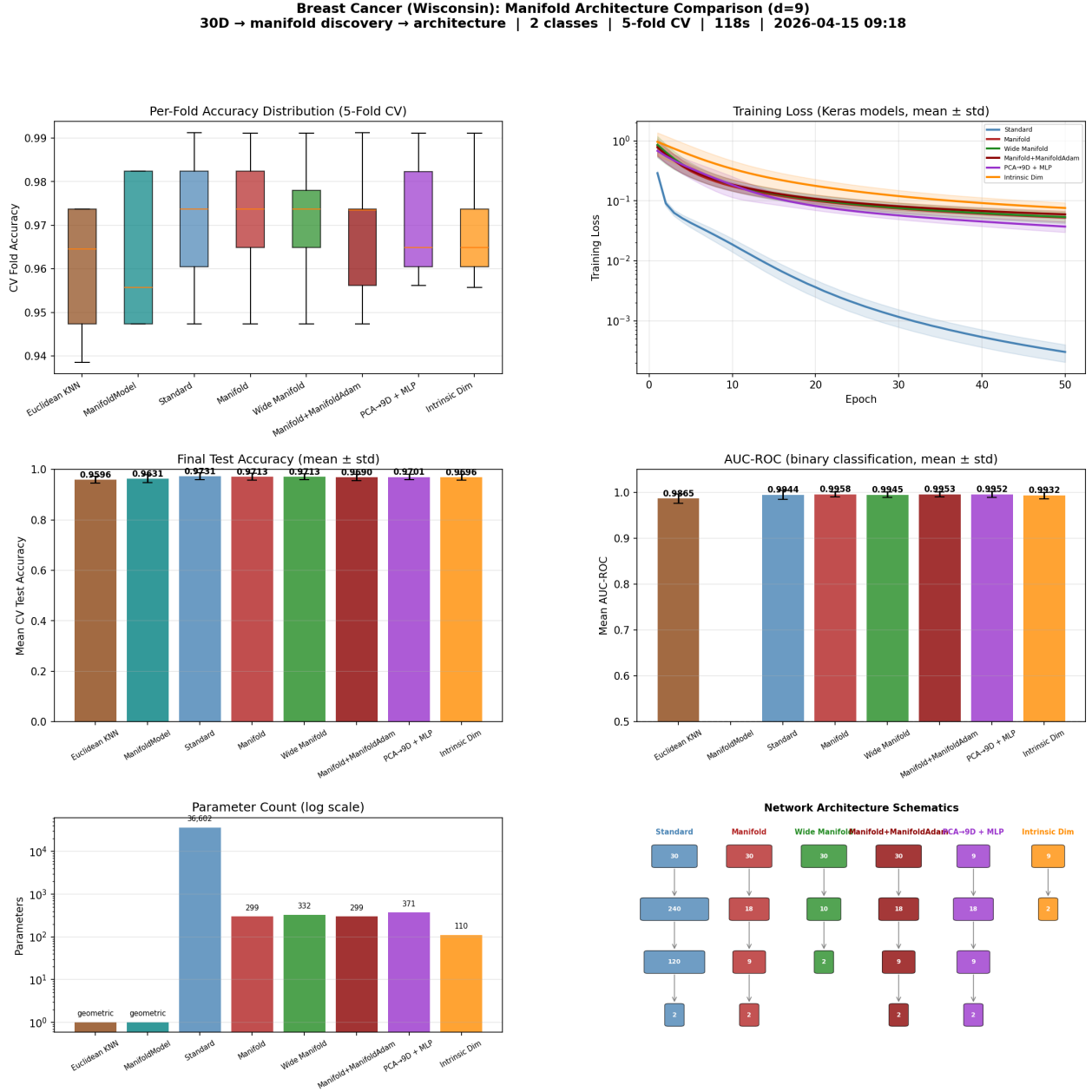
Figure 1: BREAST_CANCER manifold-informed vs. standard architecture comparison. d = 9 , 50 epochs, 3 trials.
