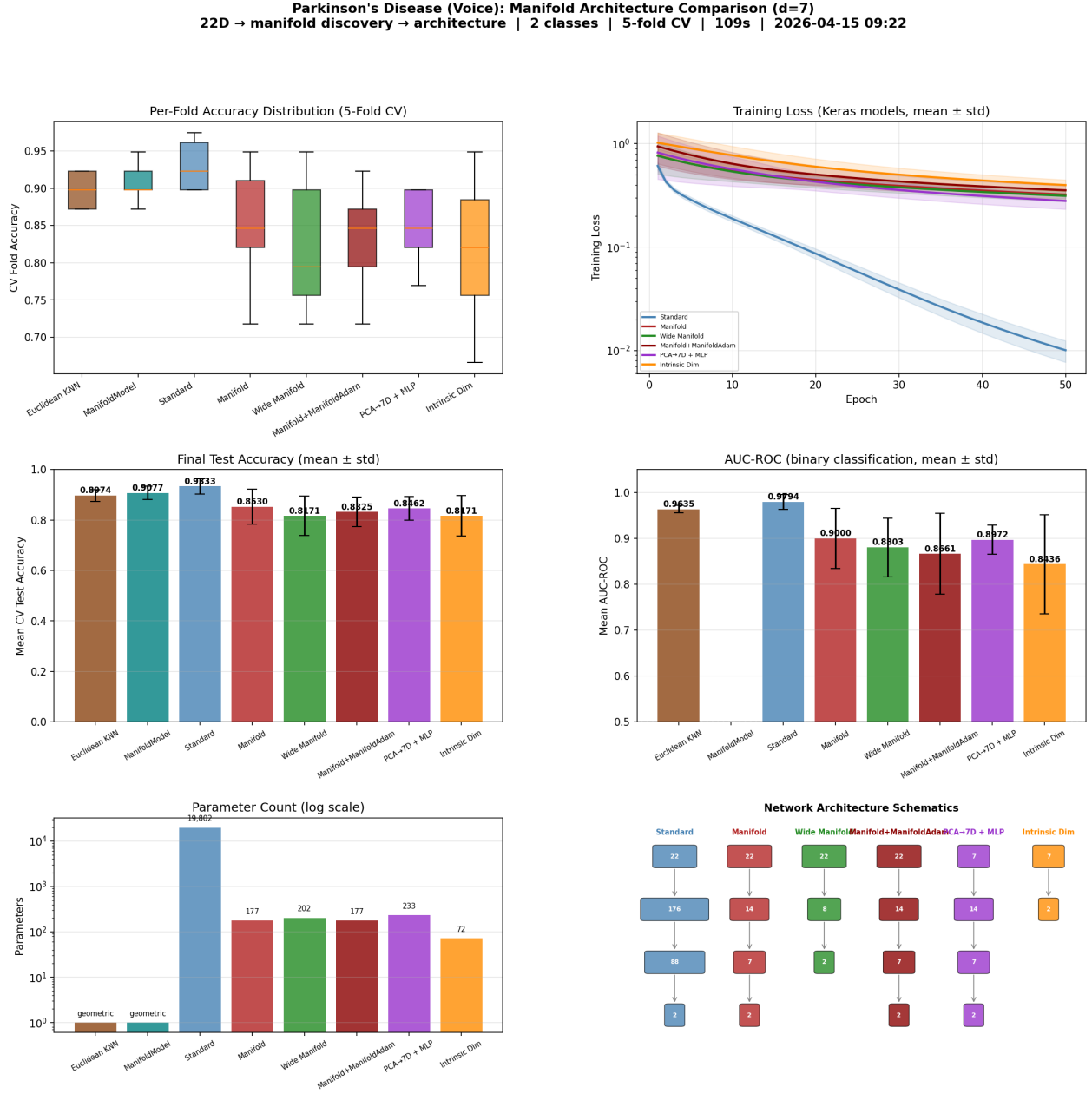
Figure 1: PARKINSONS manifold-informed vs. standard architecture comparison. d = 7 , 50 epochs, 3 trials.
