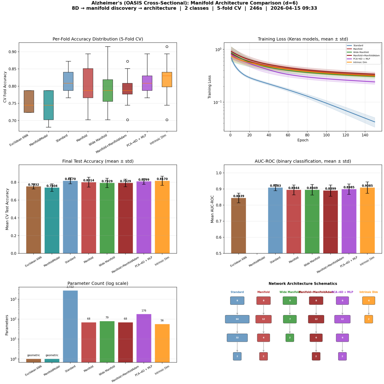
Figure 1: ALZHEIMERS manifold-informed vs. standard architecture comparison. d = 6 , 150 epochs, 3 trials.
