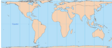
1. Behrmann
