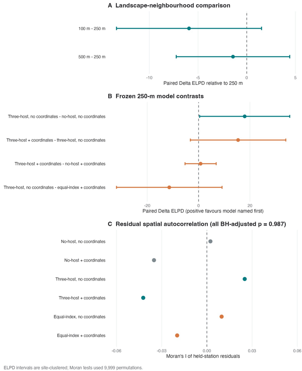
Figure S5. Whole-station transfer, scale and residual-spatial diagnostics for Koel weekly acoustic opportunity. (A) Paired change in held-station ELPD for 100- and 500-m landscape neighbourhoods relative to 250 m under the matched no-host coordinate-trend structure. (B) Frozen 250-m contrasts testing the joint host block, coordinate
