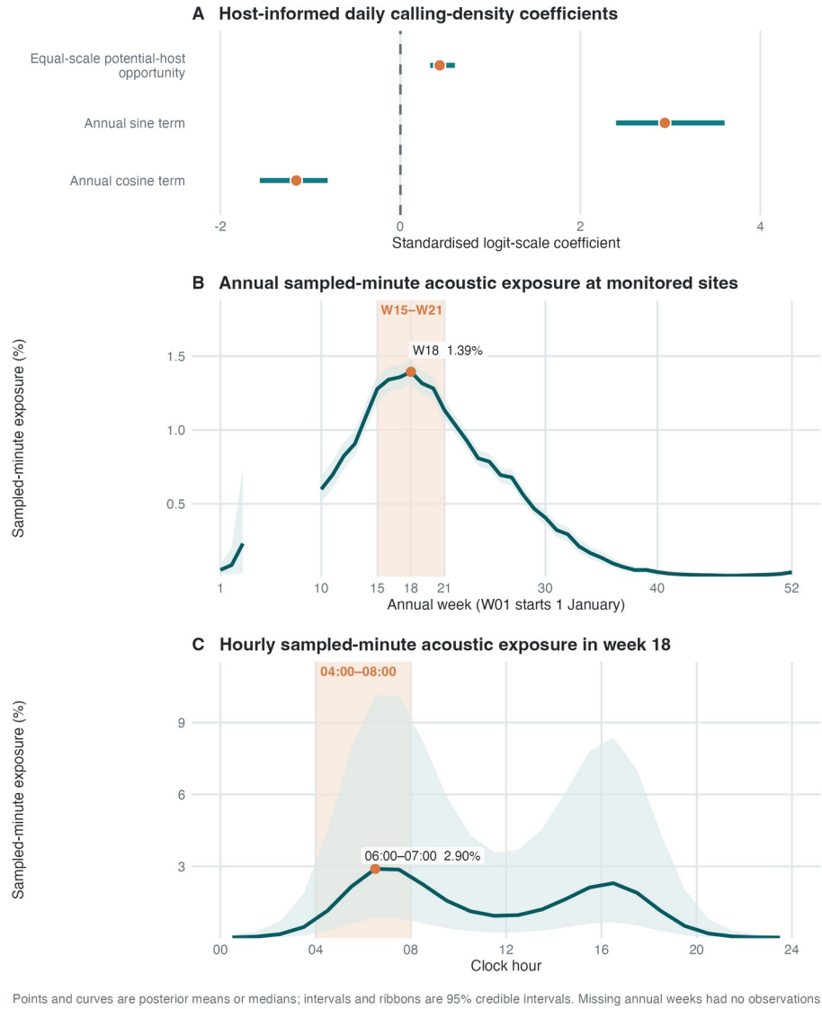
**Figure S6. Host-informed calling density and temporal pattern of sampled-minute acoustic exposure.** The fitted calling-density parameter is denoted \mu . Its zero-truncation-adjusted positive-day sampled-minute probability, \mu^+ , was combined with weekly acoustic opportunity \psi and daily detectability p to derive sampled-minute acoustic exposure, E = \psi p \mu^+ . (A) Posterior medians and 95% credible intervals for the equal-scale potential-host and annual terms in the host-informed daily calling-density branch; exact values are reported in Table S11C. (B) Annual pattern of monitored-site sampled-minute acoustic exposure under observed recording conditions. Gaps indicate weeks without observations; the pale-orange band marks W15–W21, and the orange point marks the W18 maximum. (C) Hourly sampled-minute acoustic exposure in week
