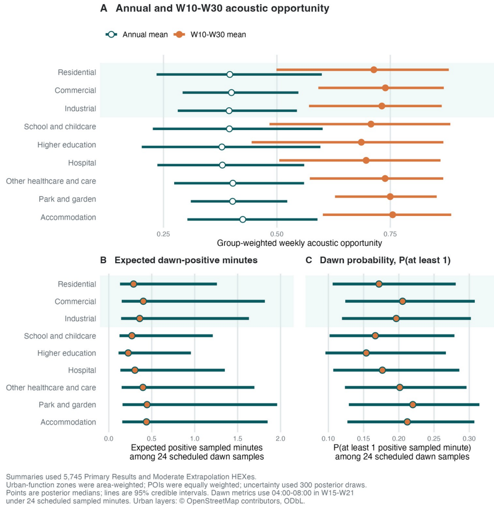
Figure S8. Modelled Koel acoustic activity overlapping mapped urban functions and sensitive places.
