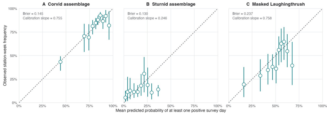
Figure S3. Whole-station calibration of the three potential-host acoustic-opportunity models. Points show observed station-week frequencies within ten equally sized groups of out-of-fold predicted probabilities for (A) the corvid assemblage, (B) the sturnid assemblage and (C) Masked Laughingthrush. The dashed line denotes perfect calibration, and vertical bars show 95% monitoring-station-cluster bootstrap intervals for the observed frequency. All predictions were generated for stations excluded from fitting. These responses quantify potential acoustic co-occurrence and do not establish brood-host use.
