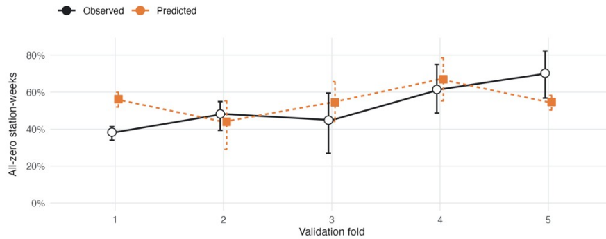
Figure S2. Whole-station validation of the retained daily-detection model. (A) Calibration of the predicted probability of at least one Koel-positive day, summarized across ten equally sized prediction groups. (B) Mean predicted number of positive days within each observed-count group; labels give the number of station-weeks. (C) Observed and predicted proportions of all-zero daily histories within each held-station fold. All predictions were generated out of fold for 31 stations and 1,500 station-weeks. Error bars are 95% monitoring-station-cluster
