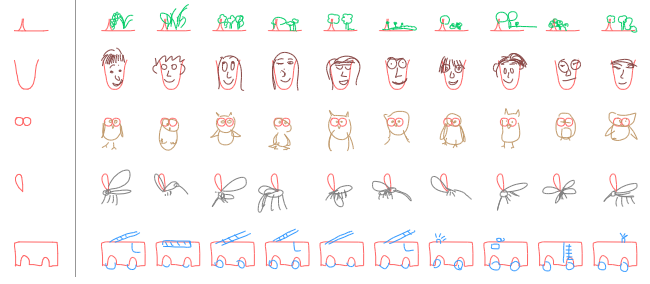
Figure 7. SketchRNN (Ha & Eck, 2017) is an example of a MDN-RNN used to predict the next pen strokes of a sketch drawing. We use a similar model to predict the next latent vector z_t .
