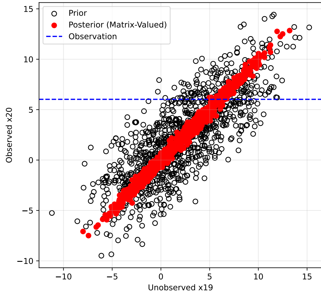
Matrix-Valued Kernel
