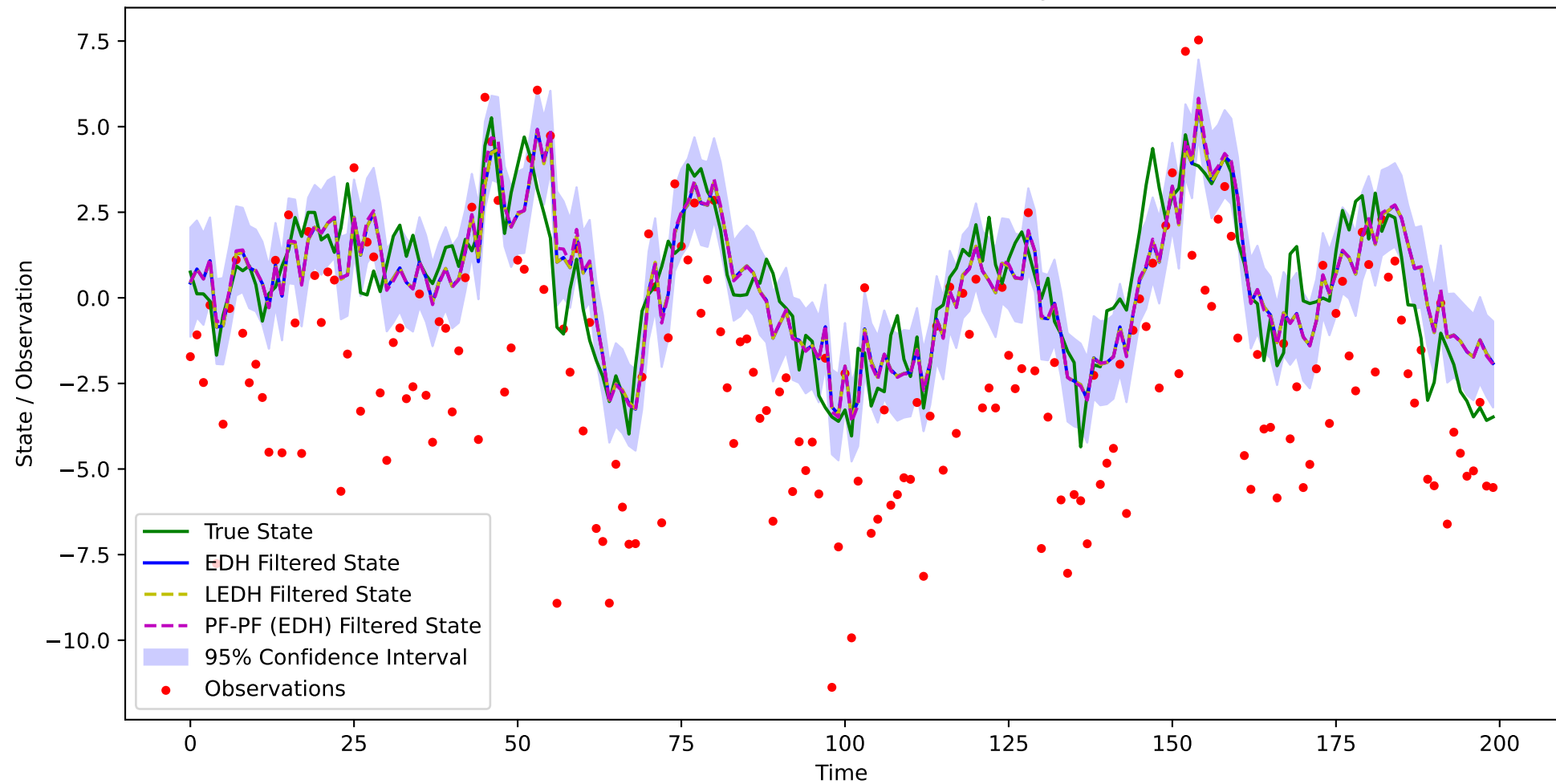
Particle Filter on 1D Stochastic Volatility Model
