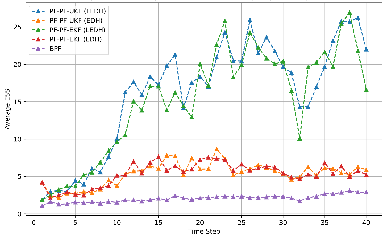
Average Effective Sample Size at Each Time Step (Figure 4 Replication)
