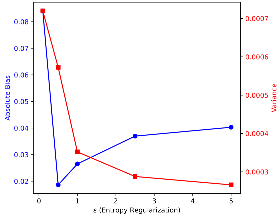
DPF Sinkhorn (Varying \varepsilon )
