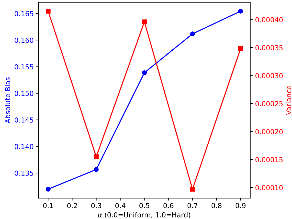
Soft Resampling (Varying \alpha )
