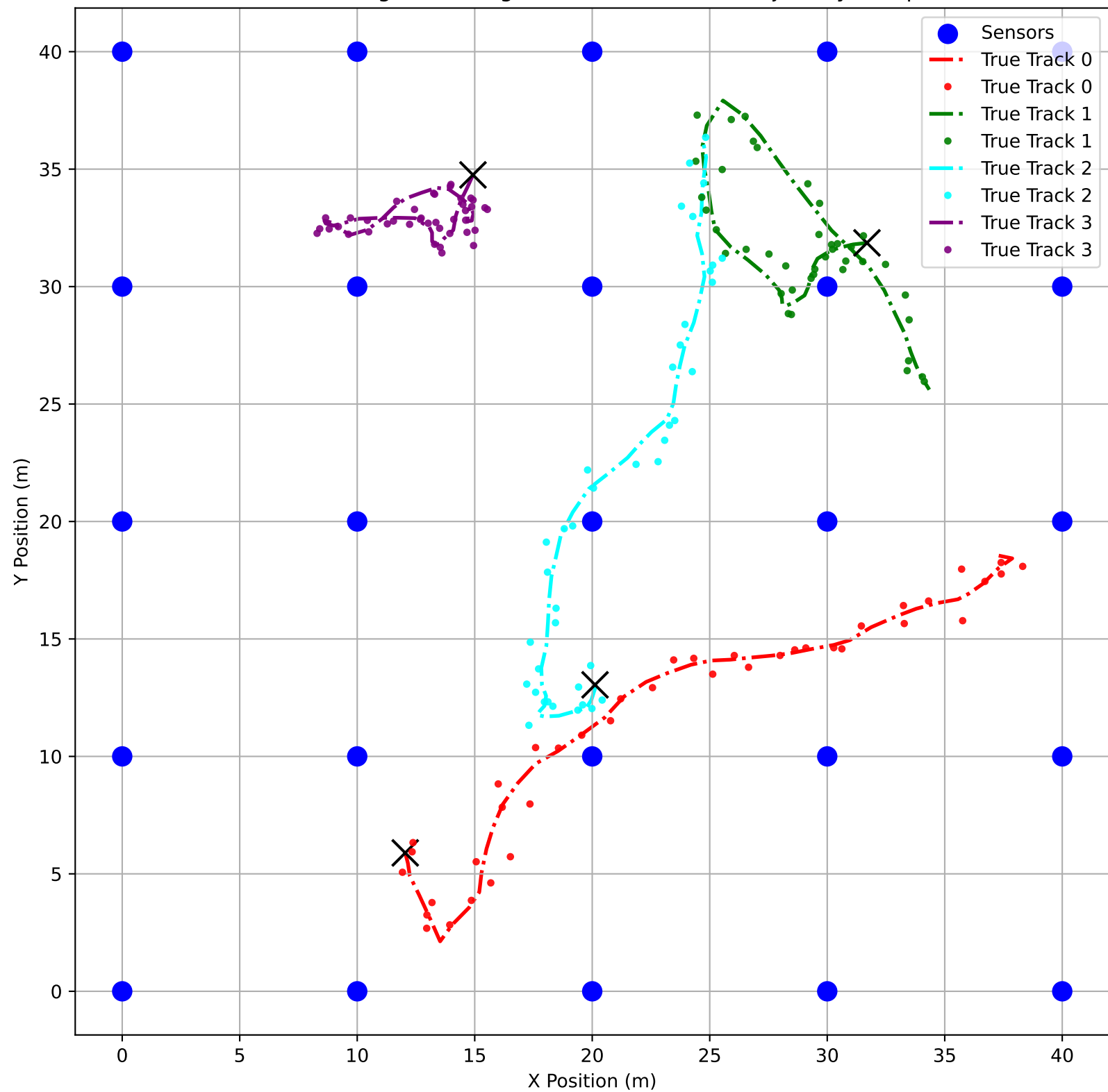
Acoustic Target Tracking - PF-PF-UKF (LEDH) Trajectory Sample
