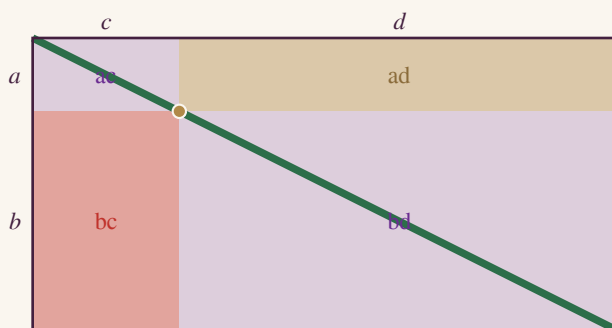
Figure 1. The dissection at the harmonic cut a = +0.25 , b = +0.75 , c = -0.50 , d = +1.50 . Complements ad (gold) and bc (crimson) are the size pair; diagonal-rectangles ac , bd (purple) are the shape pair. Here |ad|=|bc|=0.38 and ac , bd are both 2:1; the inner point sits on the diagonal.
