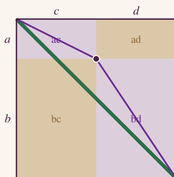
Figure 3. An off-diagonal cut (here \lambda = 1/3 ). The complements ad , bc now differ in size; the diagonal-rectangles ac , bd differ in shape; and the two corner-diagonals bend at P , peeling off the green main diagonal. One equation broke, so all three broke at once.
