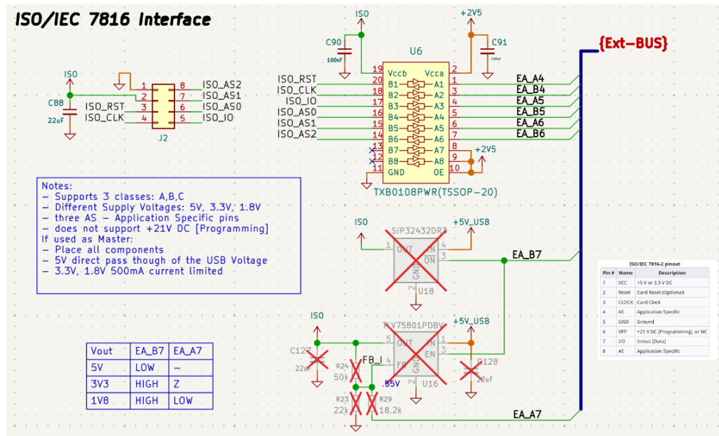
Figure 4: ISO/IEC 7816 Interface Schematic
