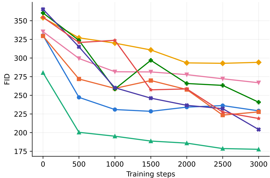
(b) FID
