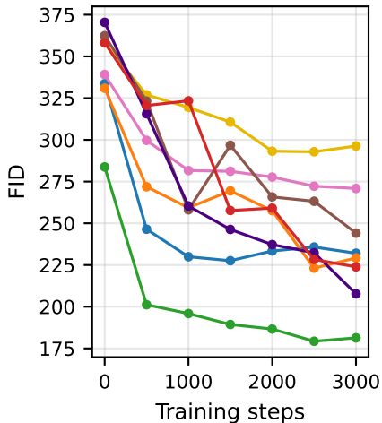
(b) FID (100 images per point)
