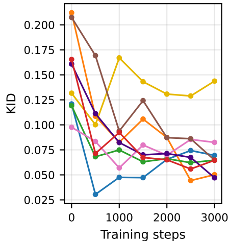
(c) KID (100 images per point)
