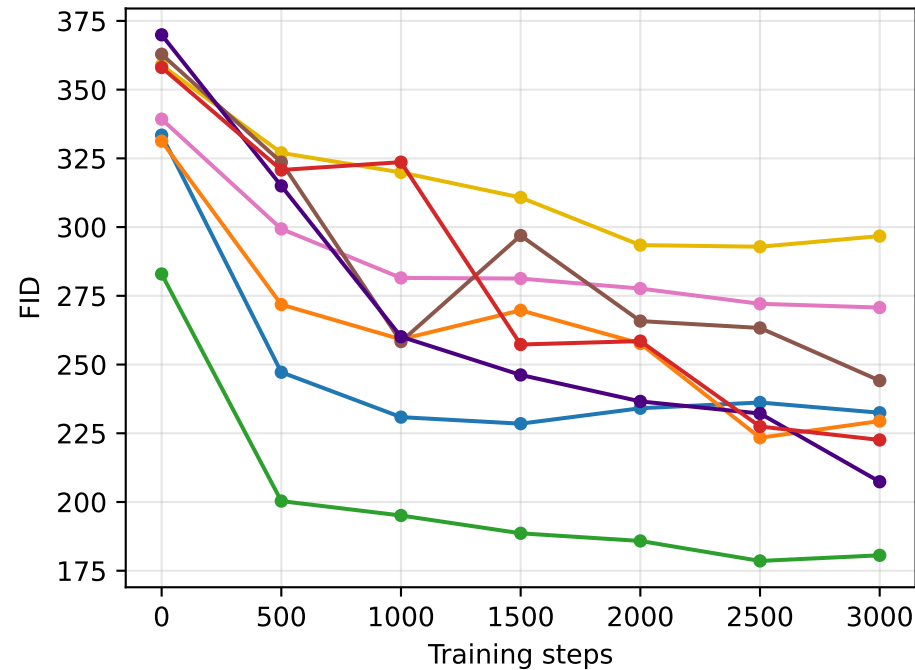
(b) FID (100 images per point)
