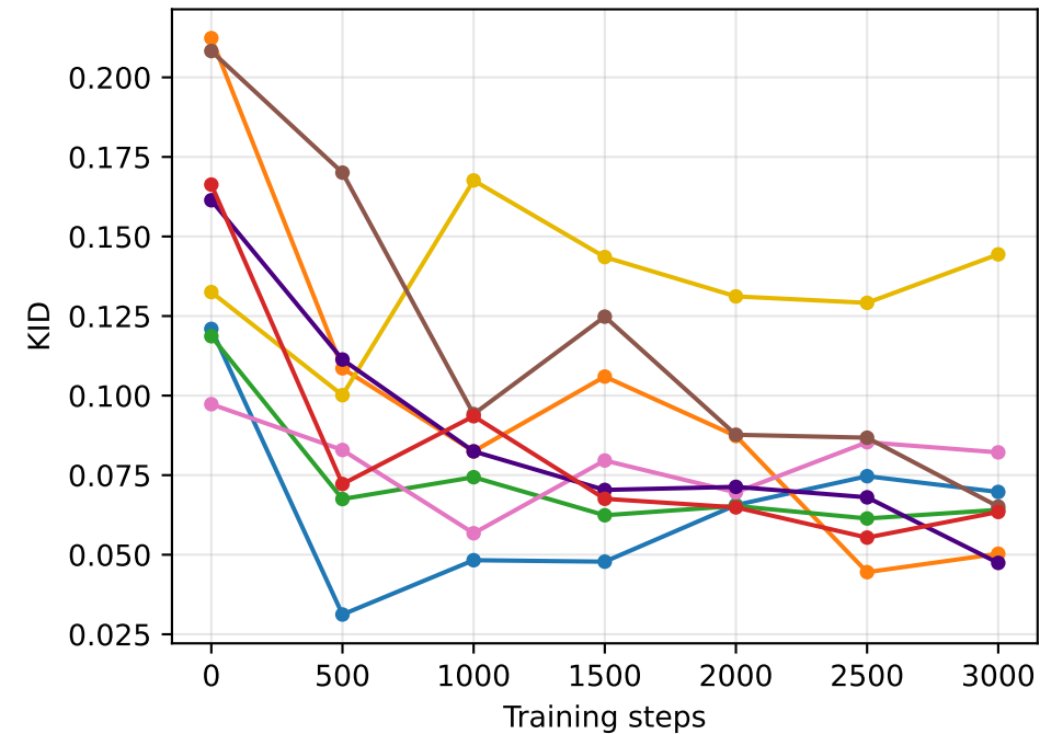
(c) KID (100 images per point)
