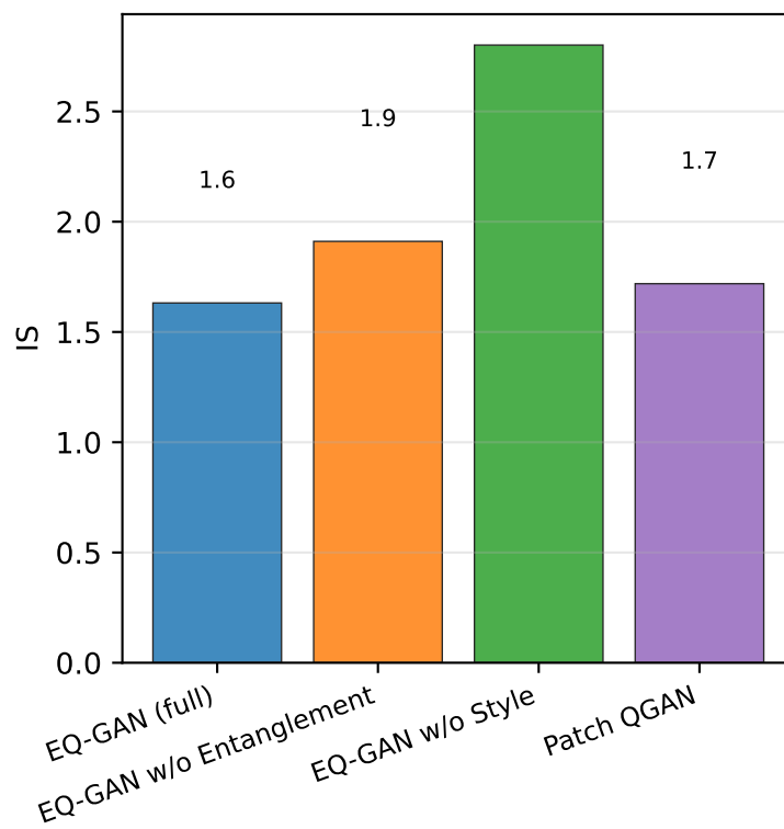
Ablation Study - FashionMNIST (50 epochs, n=5000)
