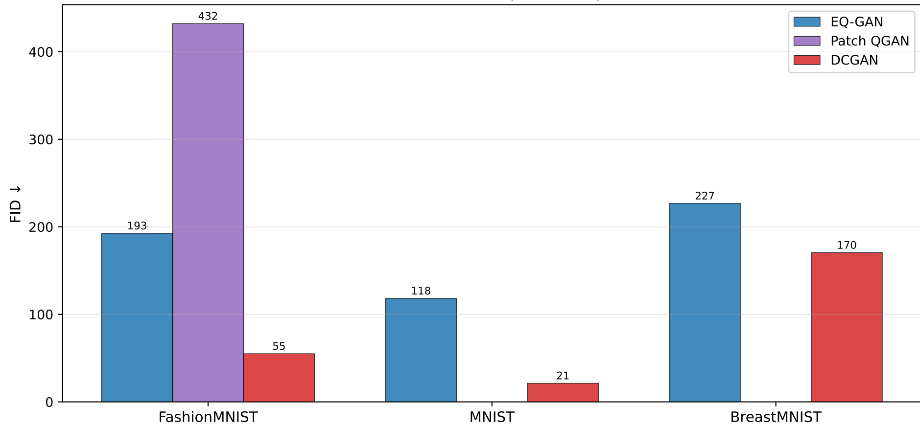
Cross-Dataset FID Comparison (Epoch 50)
