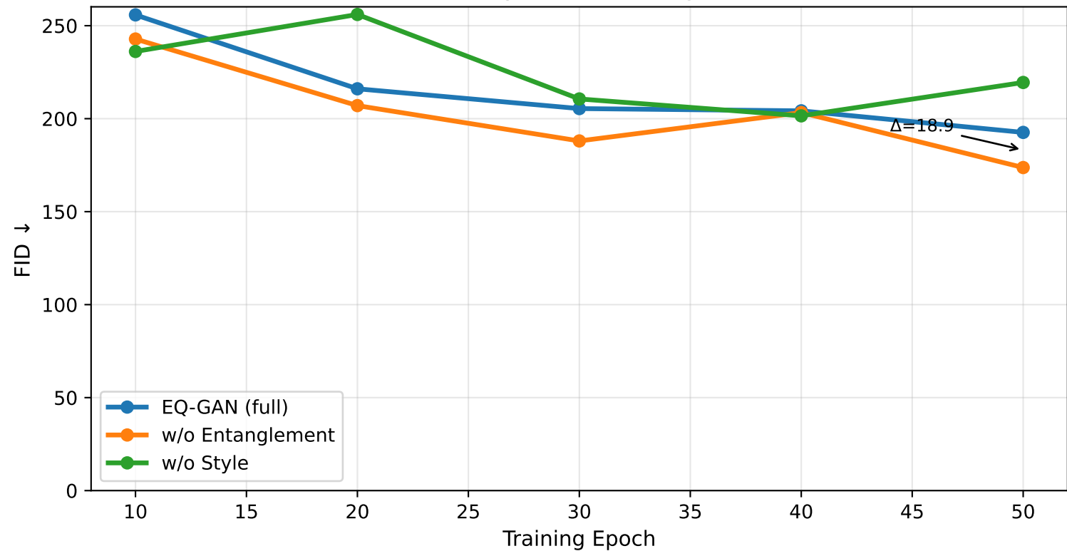
Ablation Consistency Across Training (FashionMNIST)
