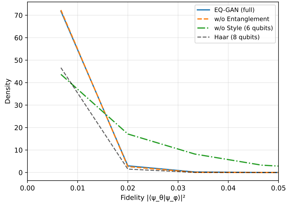
Fidelity Distribution vs. Haar (8 qubits)
