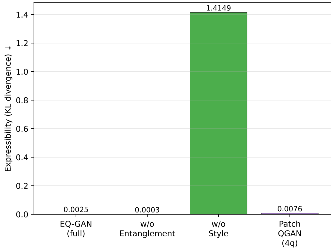
Circuit Expressibility (lower = more expressive)
