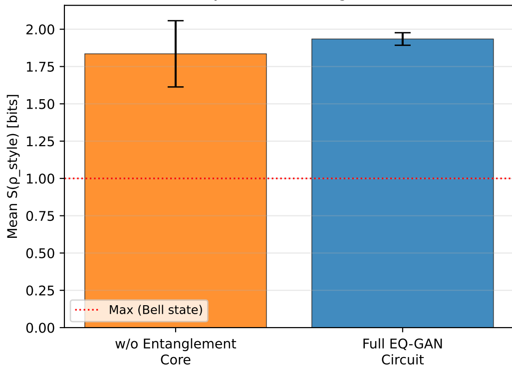
Mean Entanglement Entropy (Style \leftrightarrow Content Register)
