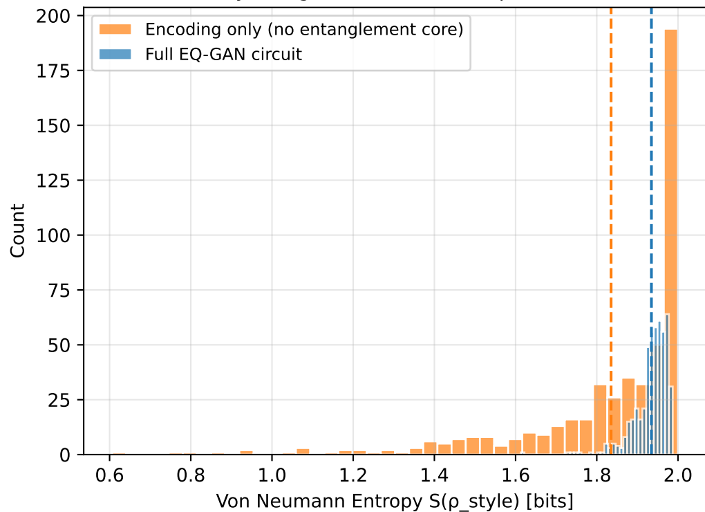
Entanglement Entropy Distribution (Style Register, 500 random params)
