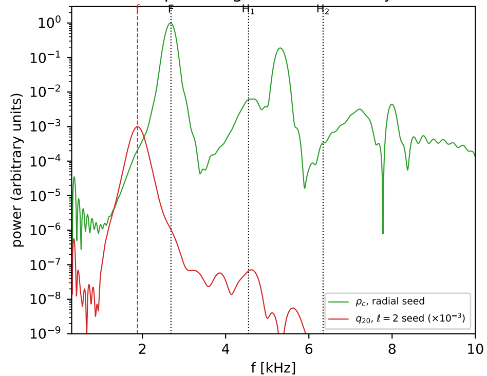
Spectra against linear theory
