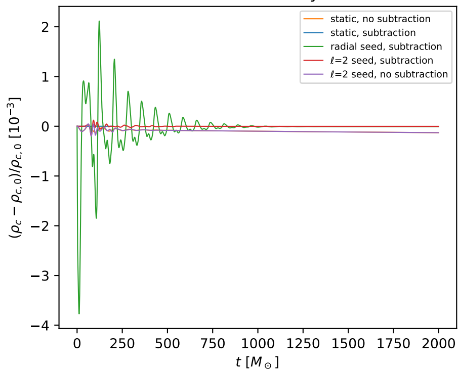
Central density
