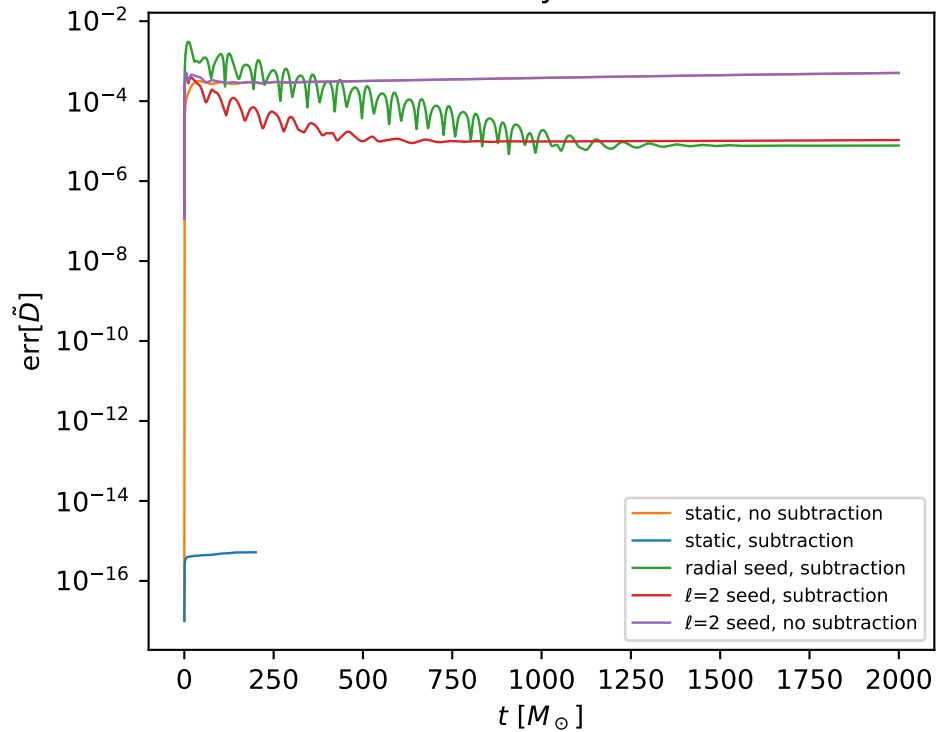
Density error
