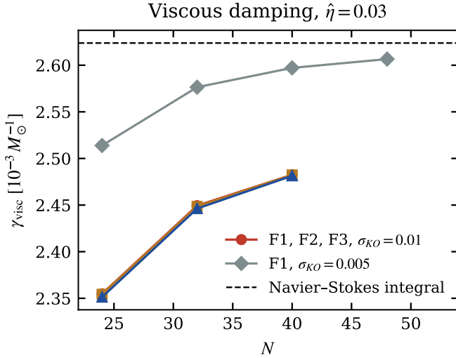
FIG. 5. Viscous damping rate of the f -mode at \hat{\eta} = 0.03 from the difference protocol, against resolution. The three Clarisse frames at \sigma_{KO} = 0.01 lie on one curve (spread 0.045% at N = 40 ). At \sigma_{KO} = 0.005 (frame F_1 , matrix pencil) the rate approaches the Navier–Stokes dissipation integral for this star (dashed).
