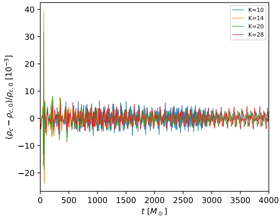
Central density, seeded \nu = 10^{-3} \sin(\pi r/R)
