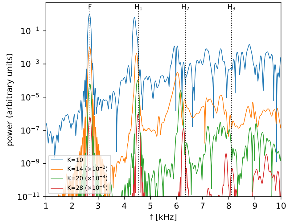
Radial spectrum vs linear theory
