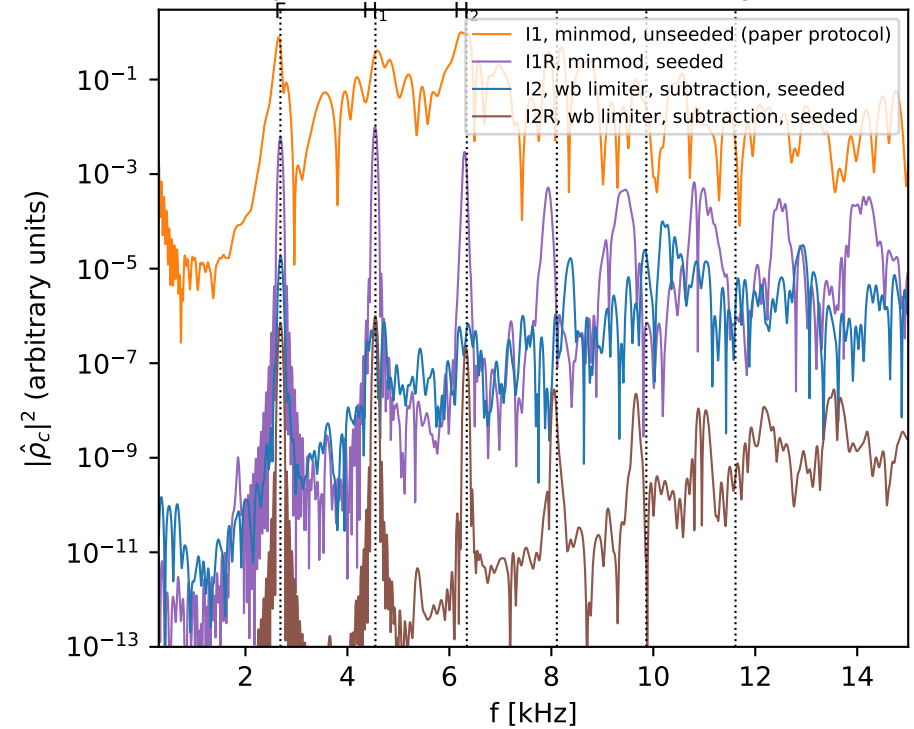
Radial spectrum of the central density, t < 4000
